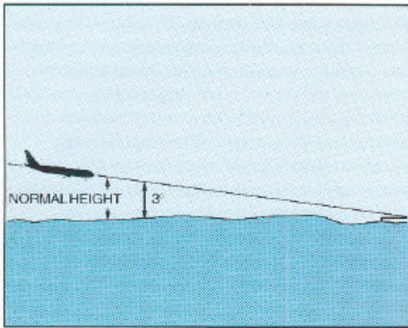
Figure 1. Nominal approach glidepath
