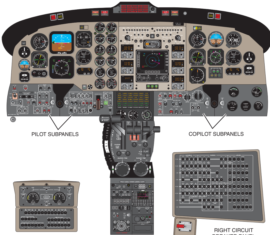
FUEL CONTROL PANEL
