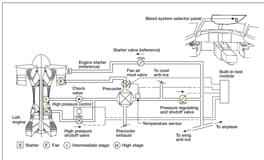
Figure 3. Bleed system
